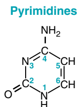
Cytosine (C)
